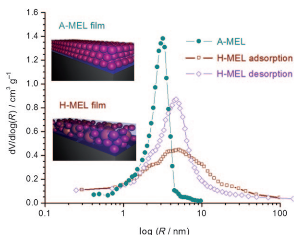
Figure 3. Mesopore radius ( R ) distribution in A-MEL and H-MEL films calculated from toluene adsorption and desorption isotherms obtained by ellipsometric porosimetry. Insets: schematics of particle packing.
